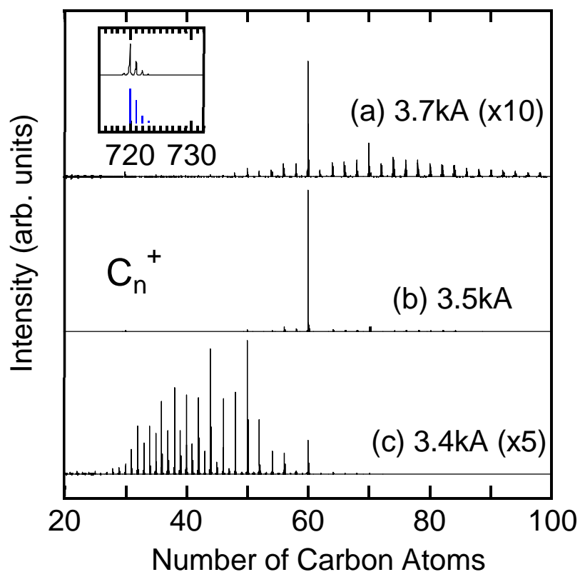
Fig. 1. Dependence of Helium gas pressure on the carbon cluster mass distribution. Insert panel is the expanded mass spectrum around C_{60} (in amu mass unit) compared to the theoretical isotopic distribution in the bottom.
