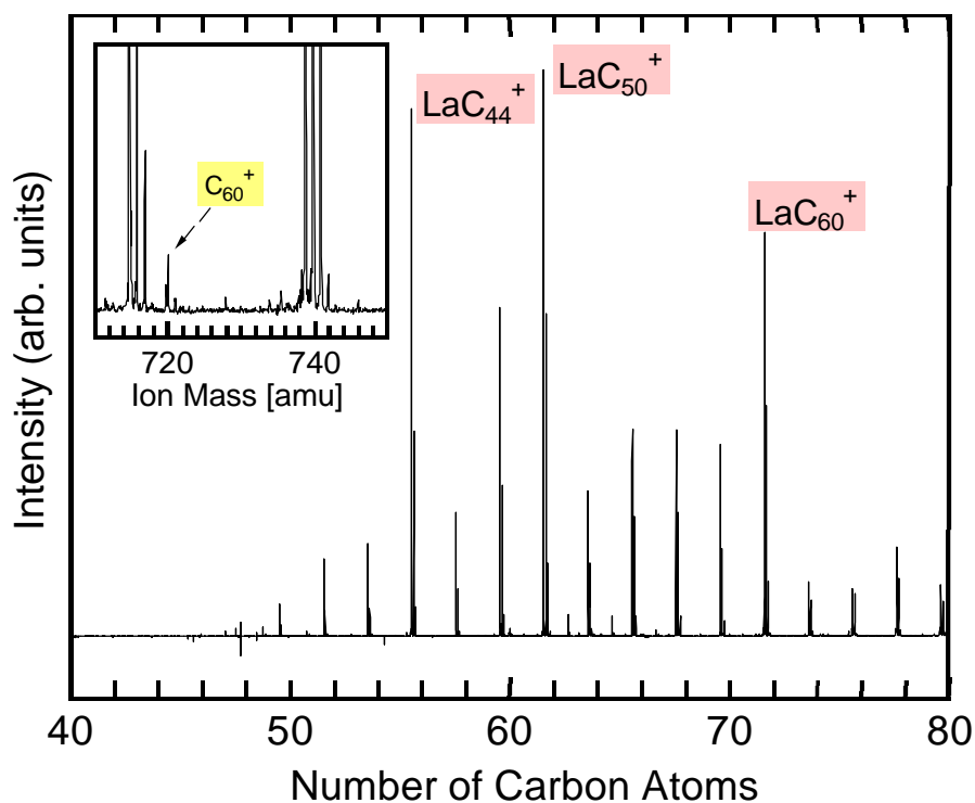
Fig.2 A mass spectrum obtained by the laser vaporization of La-carbon composite disk. interesting findings as follows. First, throughout the experiment, \text{LaC}_{44}^+ , \text{LaC}_{50}^+ and \text{LaC}_{60}^+
