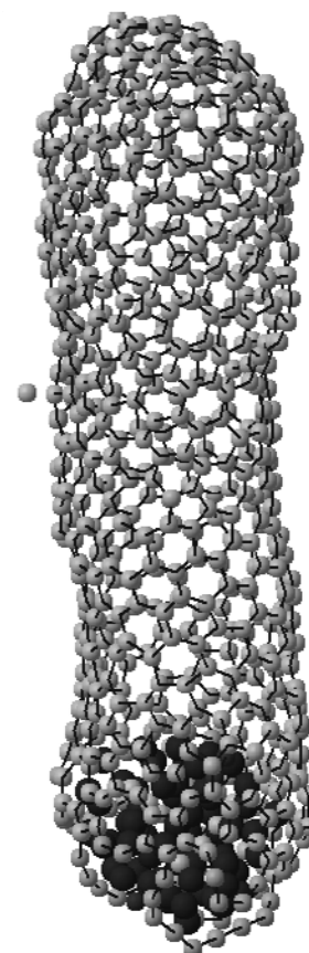
Fig. 1. Octopus mode growth from a \text{Co}_{60} cluster at 1600K. Carbon density corresponds to the atmospheric pressure.
