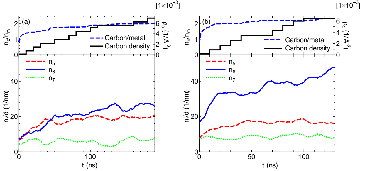
Figure 4. Structural properties of the inner SWNT growth for (a) (10, 10) and (b) (15, 6) outer SWNTs. In the bottom figures, the time histories of the number of 5, 6, and 7 membered rings ( n_5 , n_6 , n_7 ) are denoted with dashed, solid, and dotted lines, respectively. Here, d is the diameter of the outer SWNT. The top figure denotes the ratio of number of carbon atoms ( n_c ) to that of metal atoms ( n_m ) in the metal carbide cluster with the dotted lines, and the feedstock carbon density ( \rho_c ) with the solid lines.
