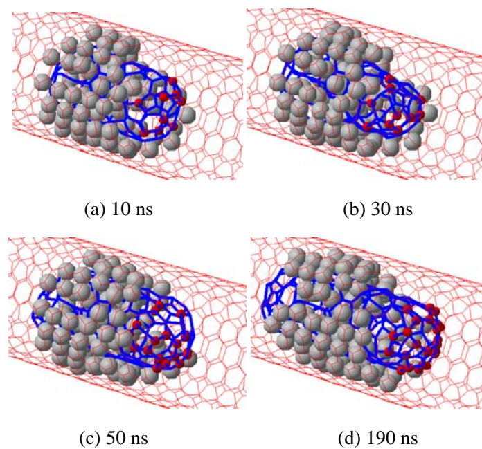
Figure 2. Trajectories of carbon atoms. The carbon atoms forming the cap at t=190 ns is denoted with red spheres.
