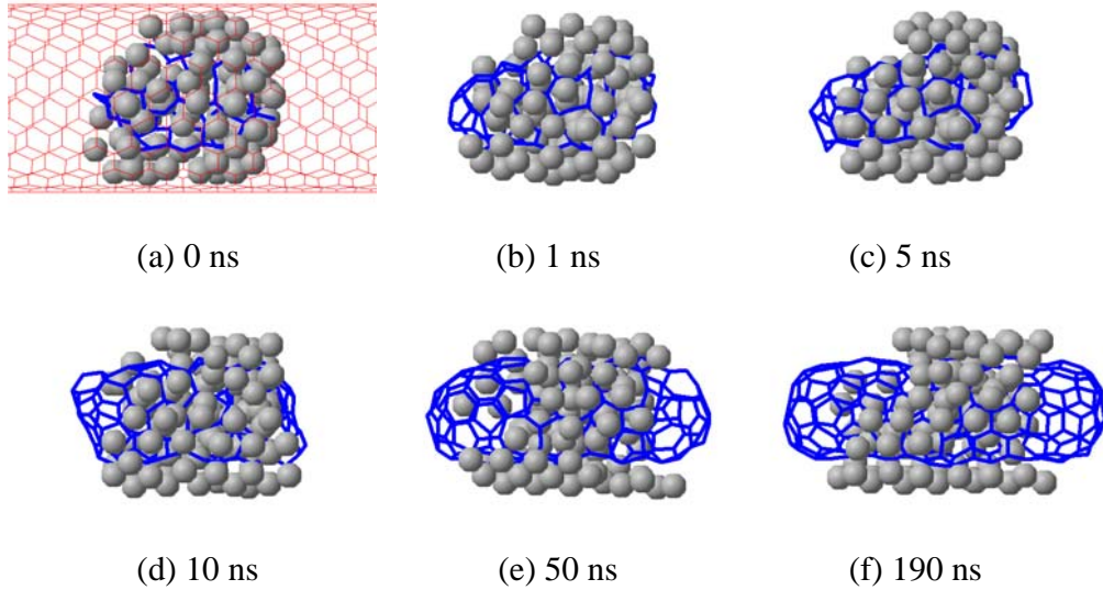
Figure 1. Growth process of an SWNT (blue) inside a template (10, 10) SWNT (red). Covalent bonds of the inner and outer SWNTs are denoted with blue and red lines. The outer SWNT is omitted for (b-f) for visual clarity.
