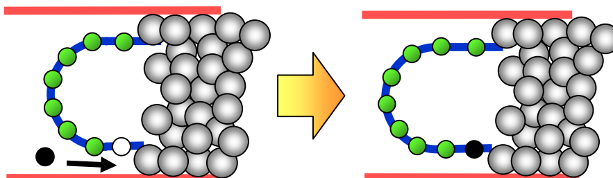
Figure 3. Schematics of inner SWNT growth process.
