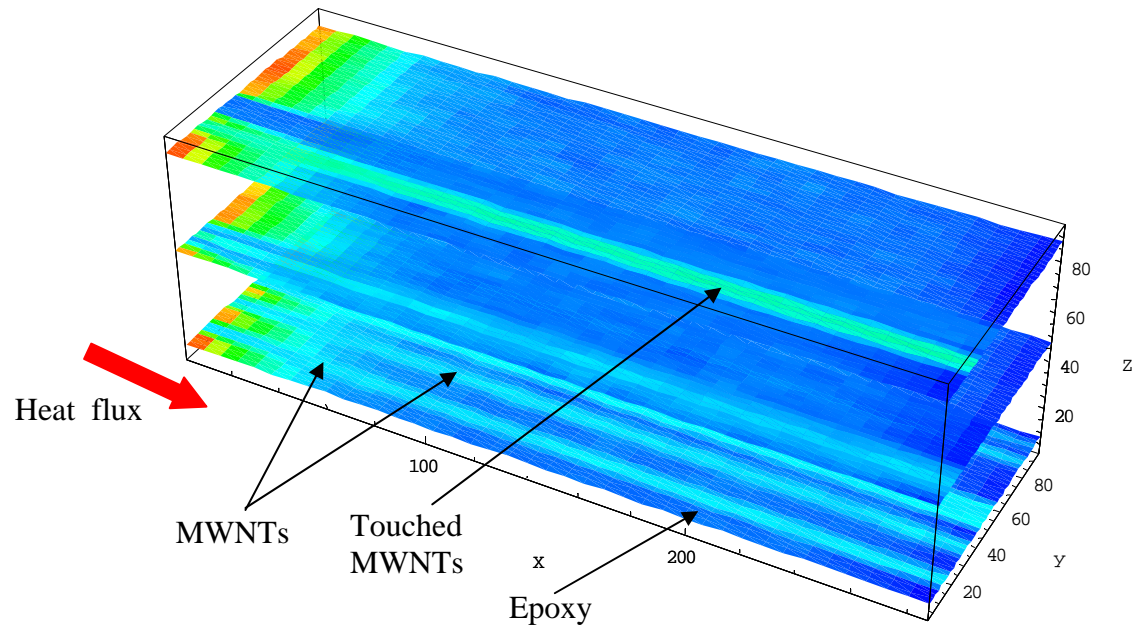
Figure 3. Heat distribution of the MWNT-epoxy composite at 20 vol% of the MWNTs parallel to the heat flux at different positions of the 288 \times 96 \times 96 grid epoxy cell. The cell is scaled by the grid unit.
