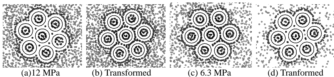
Fig. 1 Phase transformation of a small bundle of (10,10) SWNTs with hydrogen absorption Note that carbon atoms are not shown and SWNT are shown as bonds.
