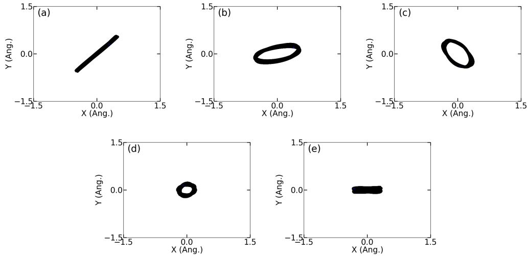
Fig. 2.11. Poincaré map for suspended case of (5,5) 23.5 nm at 500K. Each figure has 0.6 ns duration; (a) 2.2 ns, (b) 7.2 ns, (c) 12.2 ns, (d) 17.2 ns, (e) 22.2 ns.
