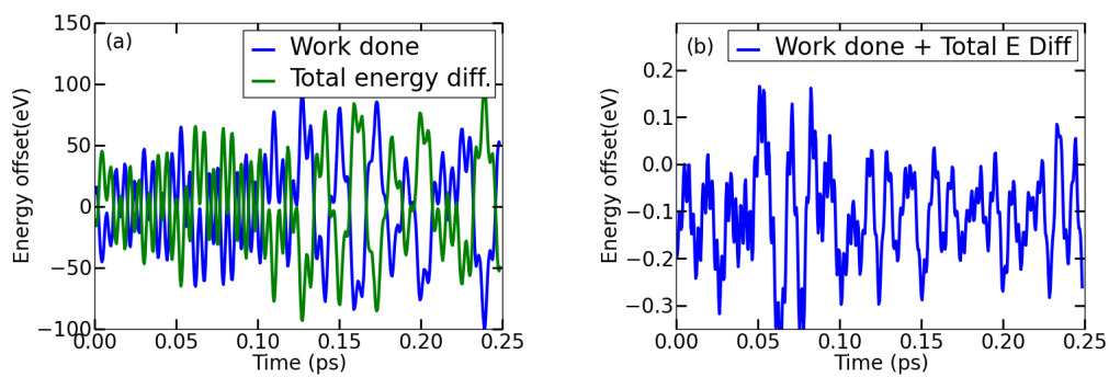
Fig. 4.3. Energy profile for analys I, (a) The work done by spring constant and energy from the given displacement of beads model, (b) sum of the work done and total energy of a lumped mass .
