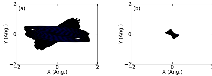
Fig. 4.9 Poincare map of tip location of (5,5) SWNT at 300K, (a) CGMD with initial condition from beads model, (b) Langevin thermostatted CGMD calculation.
