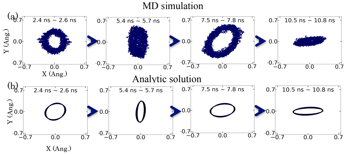
Fig. 3.4. Comparison of motion exchange in Poincaré map; (a) MD simulation and (b) analytic solution.
