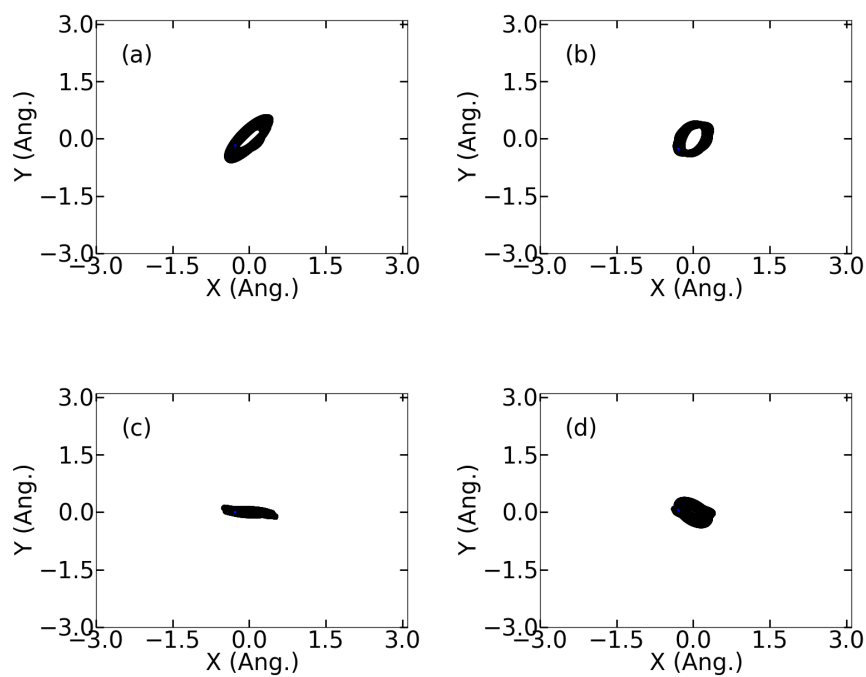
Fig. 2.6. Poincaré map after IFFT process from Fig. 2.2: (a) 1.2 ns ~ 1.8 ns, (b) 3.6 ns ~ 4.2 ns, (c) 8.4 ns ~ 9.0 ns, (d) 6.0 ns ~ 6.6 ns.
