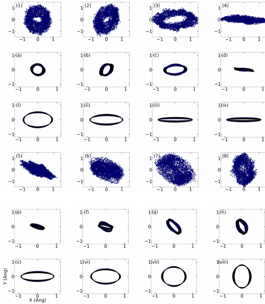
Fig. 3.6. Poincare map of (5,5) 7.6 nm case at 300 K from MD (1~8), ifft result (a~h) and analytic solution (i~viii); (1,a,i) 0.6 ns ~1.2 ns, (2,b,ii) 1.8 ns ~2.4 ns, (3,c,iii) 3 ns ~3.6 ns, (4,d,iv) 5.4 ns ~ 6 ns, (5,e,v)6.6 ns ~ 7.2 ns, (6,f,vi) 8.4 ns ~9 ns, (7,g,vii) 9.6 ns~ 10.2 ns, (8,h,viii) 10.8 ns~ 11.2 ns.
