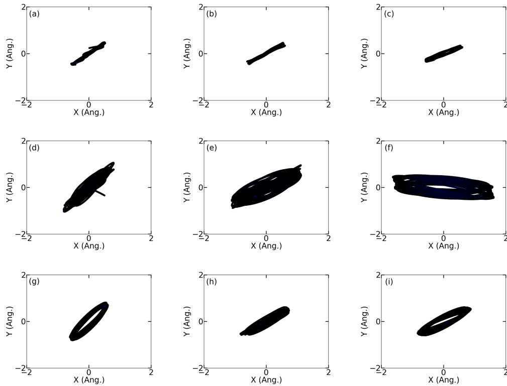
Fig.4.4. Poincaré map from MD and CGMD for free thermal vibration; MD simulation (a) 0.6 ns ~ 1.2 ns, (b) 1.8 ns ~ 2.4 ns, (c) 3.0 ns ~ 3.6 ns; CGMD modeled with 10 atoms per node (d) 0.6 ns ~ 1.2 ns, (e) 1.8 ns ~ 2.4 ns, (f) 3.0 ns ~ 3.6 ns; CGMD modeled with 60 atoms per node, (g) 0.6 ns ~ 1.2 ns, (h) 1.8 ns ~ 2.4 ns, (i) 3.0 ns ~ 3.6 ns.
