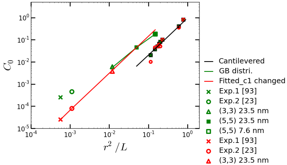
Fig. 3.10 C_0 plot for suspended case with experiment result.
