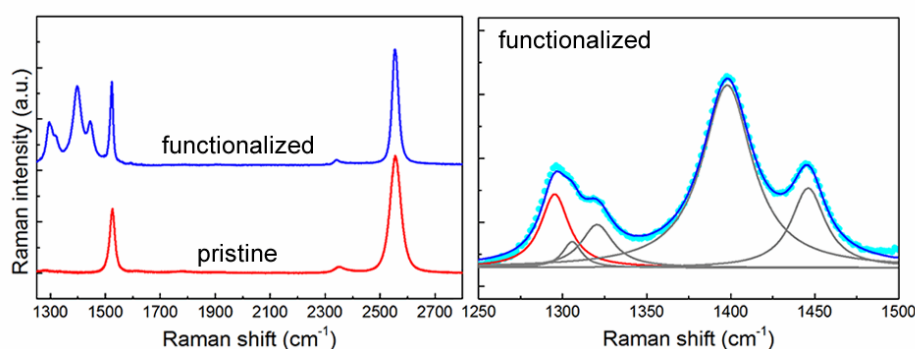
Figure S2. (Left) Typical Raman spectra of an isotopically pure ^{13}\text{C} graphene sample before (red) and after (blue) the aryl-group functionalization. (Right) Enlarged spectrum within 1250 to 1500 \text{cm}^{-1} of the ^{13}\text{C} graphene after aryl-group functionalization. Red and grey decomposed peaks indicate the newly generated defect peak in graphene and peaks from aryl groups, respectively.
