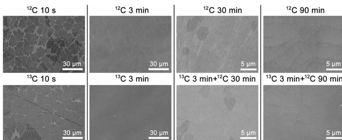
Figure S1. Comparisons of ^{12}\text{C}_2\text{H}_5\text{OH} (50 sccm) flow CVD and its equivalent ^{13}\text{C}_2\text{H}_5\text{OH} (0.4 \mu\text{L} ) no-flow CVD experiments.
