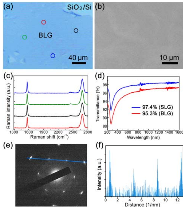
Figure 1. (a) Optical microscope (OM) image of a BLG film on a Si substrate with a 100-nm-thick SiO 2 layer. (b) SEM image of as-grown ethanol-derived BLG film on a Cu foil. (c) Typical Raman spectra of BLG measured from four random spots in (a). (d) Transmittance spectra of a transferred BLG film (red), and a reference SLG film (blue). (e) SAED pattern of a bilayer graphene domain, which shows clear six-fold symmetry. (f) The spot intensities along the blue line in (e).
