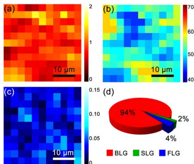
Figure 2. Scanning Raman maps of ethanol-derived BLG for (a) I_{2D}/I_G , (b) FWHM of the 2D-band and (c) I_D/I_G . (d) The corresponding pie chart of graphene coverage for BLG, SLG and FLG in the ethanol-derived BLG film.
