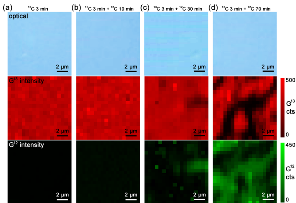
Figure 6. OM images and scanning Raman maps of ^{12}\text{C} and ^{13}\text{C} G-band peaks for the SLG areas in ethanol-derived graphene samples grown by: (a) 3 min ^{13}\text{C}_2\text{H}_5\text{OH} ; (b) 3 min ^{13}\text{C}_2\text{H}_5\text{OH} followed by 10 min ^{12}\text{C}_2\text{H}_5\text{OH} ; (c) 3 min ^{13}\text{C}_2\text{H}_5\text{OH} followed by 30 min ^{12}\text{C}_2\text{H}_5\text{OH} ; and (d) 3 min ^{13}\text{C}_2\text{H}_5\text{OH} followed by 70 min ^{12}\text{C}_2\text{H}_5\text{OH} . All ^{13}\text{C}_2\text{H}_5\text{OH} trials were conducted by no-flow CVD with 0.4\ \mu\text{L} ^{13}\text{C}_2\text{H}_5\text{OH} , whereas all ^{12}\text{C}_2\text{H}_5\text{OH} trials were conducted with flow CVD of 50\ \text{sccm} ^{12}\text{C}_2\text{H}_5\text{OH} . Clear substitutions of isotopic graphene flakes are observed in (c) and (d).
