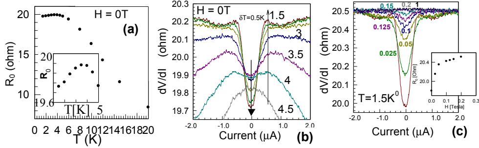
Fig. 3: Electrical properties of the sample with the partial Au-end junction. (a) R_0 as a function of the temperature. Inset : Enlarged view of the main panel for 1.5\text{K} \leq T \leq 5\text{K} . (b) Differential resistance as a function of the current for different temperatures. (c) Differential resistance as a function of the current for different magnetic fields. Inset: R_0 as a function of the magnetic field.
