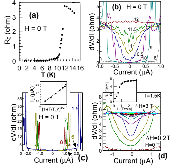
Fig. 2: Electrical properties of the sample with the entire Au-end junction. A residual resistance of < 1 \Omega has been subtracted in the figures [20]. (a) The zero-bias resistance ( R_0 ) as a function of the temperature at zero magnetic field ( H = 0 \text{ T} ). (b)(c) The differential resistance as a function of the current for different temperatures > T_c (b) and < T_c (c). The numbers on each curve denote the temperatures in Kelvin. The critical currents ( I_c ) were identified in contradiction to [4], although the slight resistance increases due to the residual resistances exist in the large current regions even in a superconductive state (c). We defined the current, at which an abrupt resistance increase appears, as I_c . The presence of resistance oscillations in the larger current regions is consistent with [4, 13] (interpreted as a phase slip). Inset of (c): I_c , which corresponds to the current values indicated by arrows in the main panel, as a function of the temperature. I_c was normalized for the Ginzburg-Landau behavior of I_c . The solid line is provided just to eyes. (d) The differential resistance as a function of the current for different magnetic fields. The number on each curve denotes the magnetic field (in Tesla) that was applied perpendicular to the tube axis. Inset: R_0 as a function of the magnetic field.
