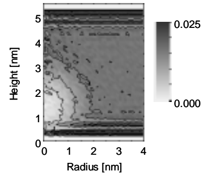
Figure 10 Equilibrium vapor bubble shape for P5 [11].
