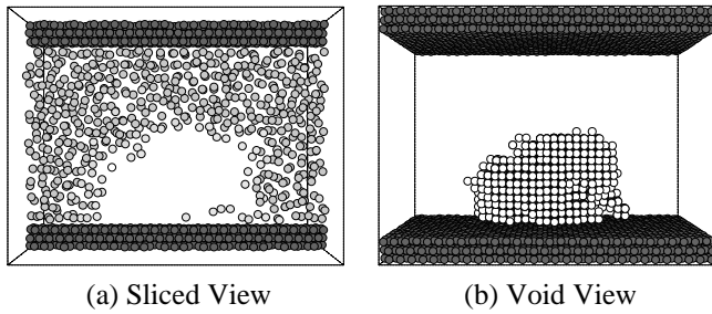
Figure 3 A snapshot of a vapor bubble at 2100 ps for E3.
