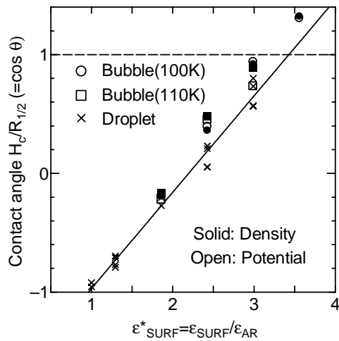
Figure 9 Contact angle correlated with \varepsilon^*_{SURF} .
