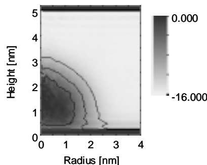
Figure 8 Two-dimensional potential distribution for E3.
