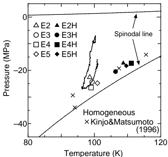
Figure 6 Pressure and temperature variations.
