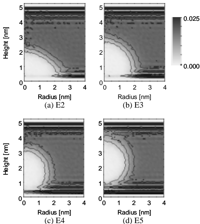
Figure 7 Two-dimensional density distributions.
