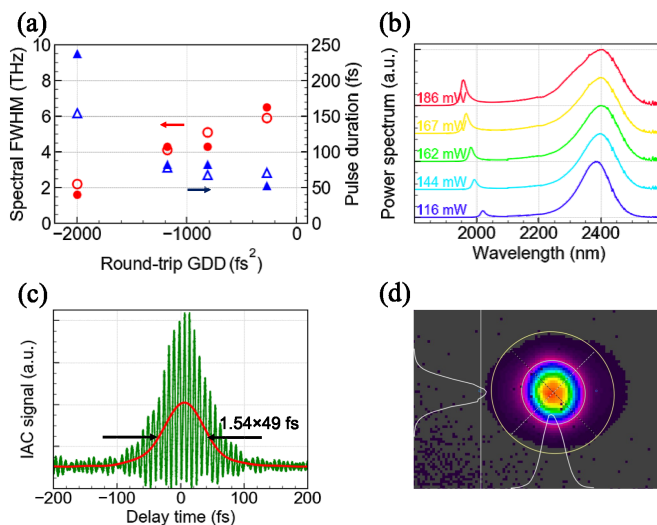
Fig. 3. CW mode-locking properties of our Cr:ZnS laser using SWCNT-SA: (a) pulse duration and spectral FWHM for varied round-trip GDD (the filled markers are for a 2.5 % OC and the blank markers are for a 10 % OC); (b) power spectrum measured for varied output power; (c) green: the measured interferometric auto-correlation, red: the retrieved intensity autocorrelation; and (d) the measured spatial beam profile (the white curves represent the Gaussian intensity distribution intersected horizontally and vertically).
