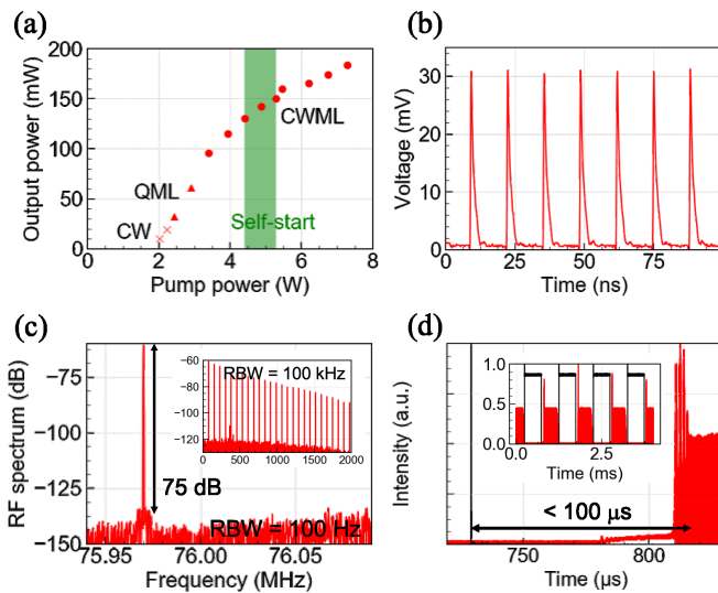
Fig. 2. Output properties of Cr:ZnS laser oscillation: (a) pump power dependence of the output power, where \times represents cw oscillation, \blacktriangle represents Q-switched mode-locking, and \bullet represents cw mode-locking; (b) oscilloscope trace of the pulse train; (c) the RF spectrum measured with RBW of 100 Hz (inset: the RF spectrum of 2-GHz span measured with RBW of 100 kHz); and (d) transient output power (red) showing the build-up process of the mode-locking, measured by modulating the cavity loss (black) at 1 kHz.
