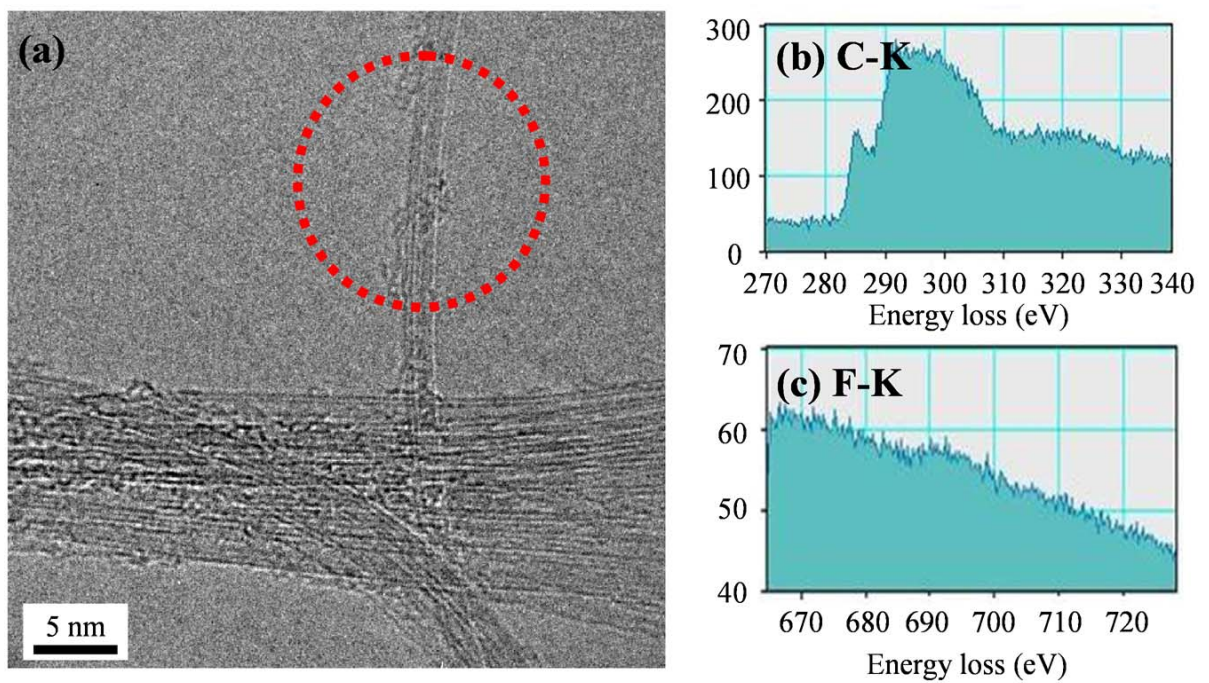
Figure 2 (a) TEM image of a single fluorinated DWNT and its corresponding electron energy loss spectra for (b) C-K and (c) F-K edges.
