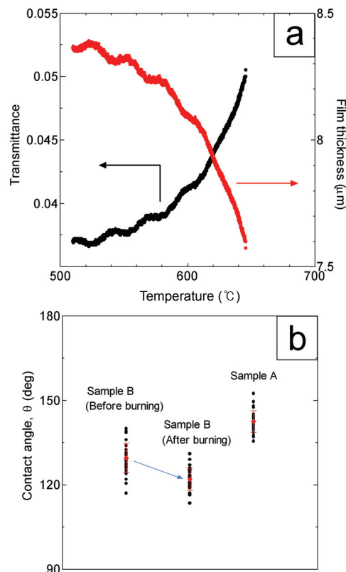
Fig. 3. (a) Measured transmittance of the incident light (left ordinate) and estimated corresponding film thickness (right ordinate) during heating from 500 to 645 ^\circ C.
