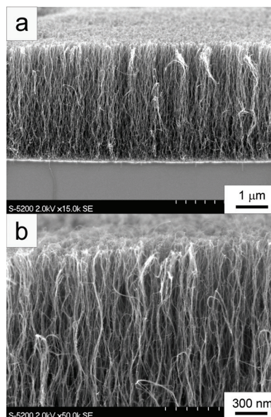
Fig. 1. Typical FE-SEM images of the VA-SWNT film grown on a fused quartz substrate. (a) Whole image of the film cross-section and (b) its magnification including the top surface.
